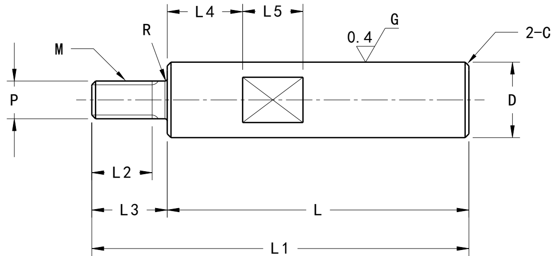
Front view Scale: 2:1
