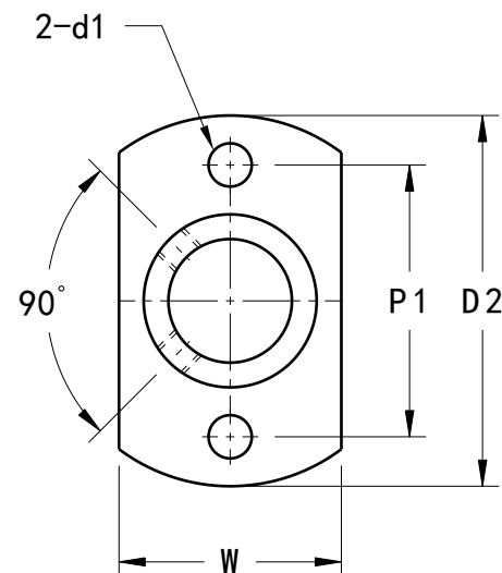
III (D3~15) Front view[2] Scale: 3:2
