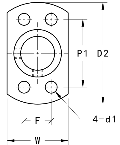
III (D16~50) Front view Scale: 3:2
